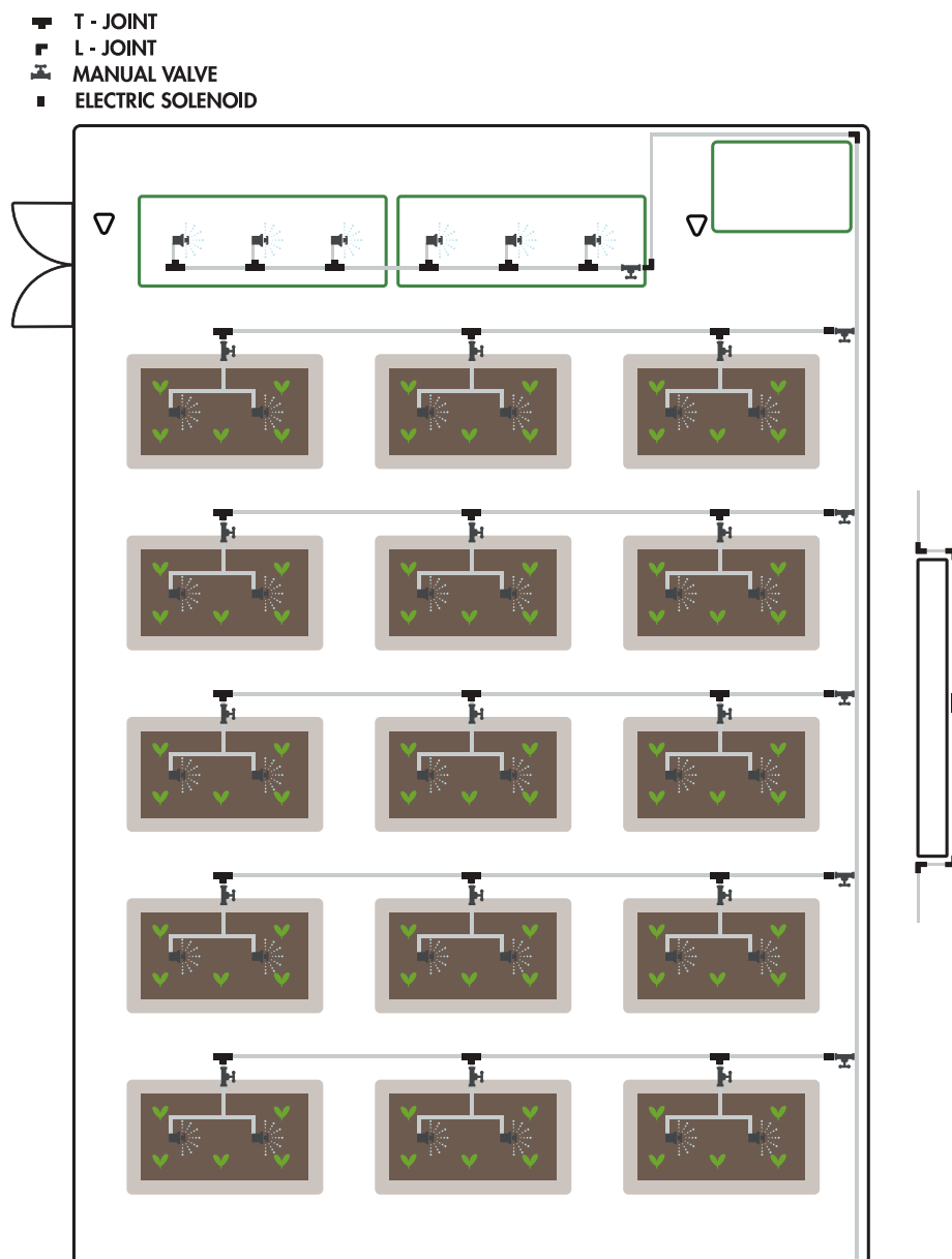
Overview of irrigation layout in Fengshan Aspen RN Community Garden
